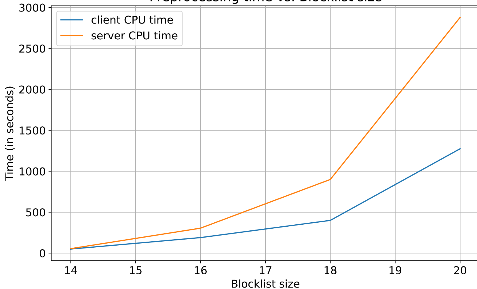
Preprocessing time vs. Blocklist size
